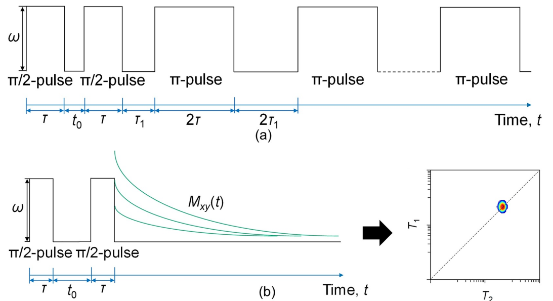
Figure B1. The variation of \omega_y(t) with time t is utilized to simulate the SR-CPMG pulse sequence: (a) the simulated SR-CPMG pulse sequence; (b) the modified SR-CPMG pulse sequence to simulate 2D T_1 - T_2 map.
