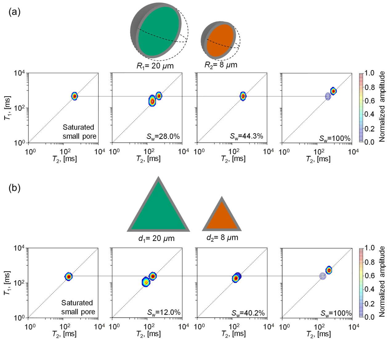
Figure 7. The simulated evolution of 2D T_1 - T_2 map of (a) dual-spherical and (b)-triangular-shaped pore system during the imbibition process.
