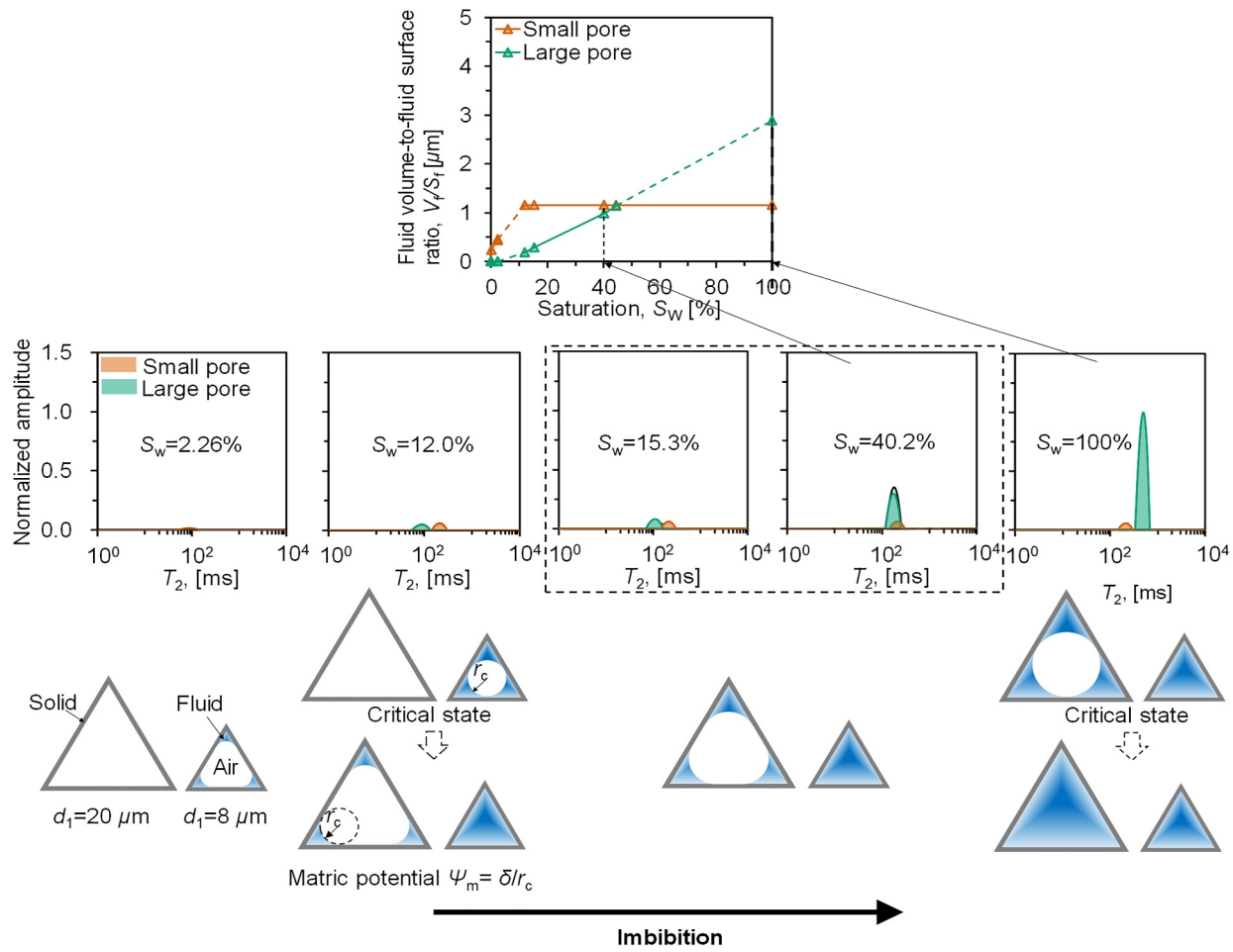
Figure 5. The simulated evolution of T_2 -distribution and variation of V_f/S_f of dual-triangle-shaped pore system during the imbibition process.
