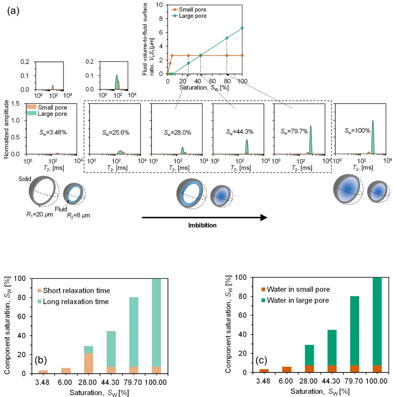
Figure 4. (a) The simulated evolution of T_2 -distribution and variation of V_p/S_f of dual-spherical pore system during the imbibition process; (b) the water partitioning of the dual-spherical pore system revealed by different relaxation time peaks; (c) the pore water dynamic distribution of the dual-spherical pore system.
