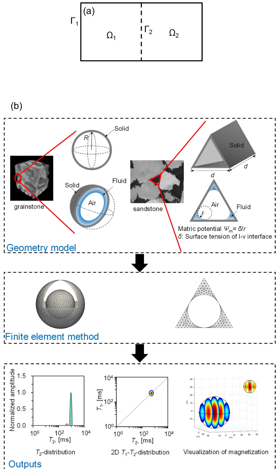
Figure 2. Description of the simulation framework of NMR response: (a) Scenario of confined unsaturated pore space; (b) The typical workflow for simulation of the NMR relaxation process in porous media.
