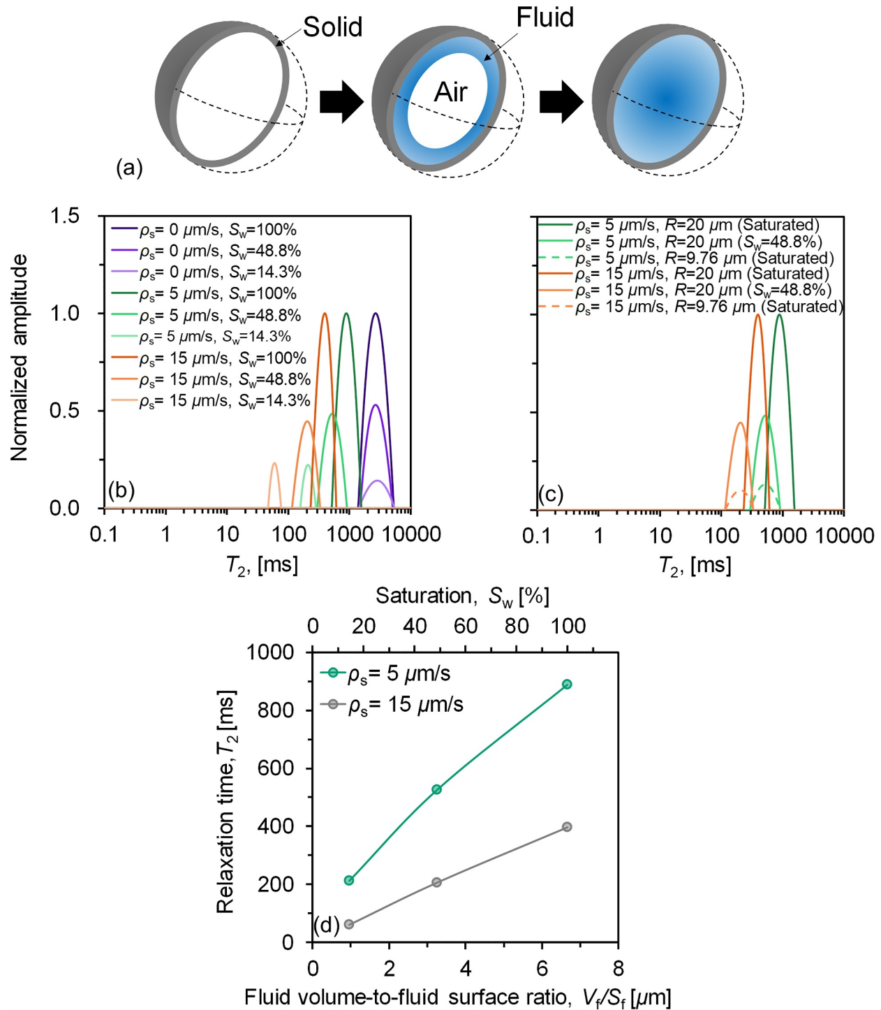
Figure 3. The imbibition process of the single spherical pore and its simulated NMR response: (a) the imbibition process of the single spherical pore; (b) the simulated T_2 -distribution of the single spherical pore with different surface relaxivity under different saturation states; (c) the unsaturated spherical pore display short relaxation times akin to saturated smaller spherical pore; (d) the comparison of the variation of peak T_2 time and V_f/S_f of the single spherical pore during the imbibition process.
