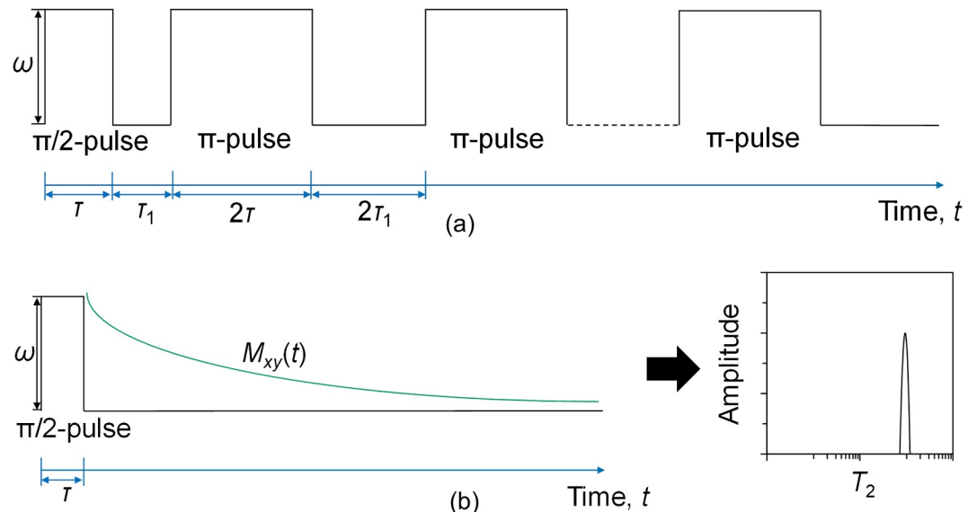
Figure A1. The variation of \omega_y(t) with time t is utilized to simulate the CPMG pulse sequence: (a) the simulated CPMG pulse sequence; (b) the modified CPMG pulse sequence to simulate T_2 -distribution.
