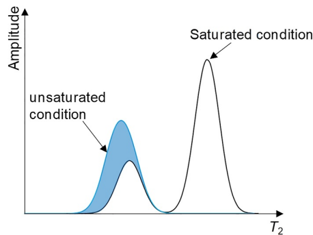
Figure 1. Comparative NMR T_2 -distribution in unsaturated and saturated porous media (the shaded blue area signifies the reduced amplitude of short relaxation times from unsaturated to saturated conditions).
